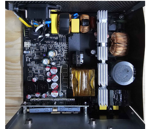
PSU Internals
