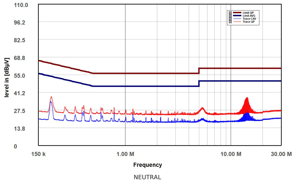
Thermaltake Dockpower FI 1000W (TT10003418) Neutral
