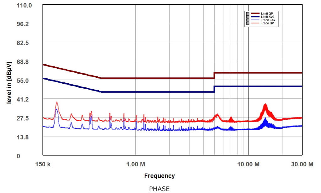
Thermaltake Dockpower FI 1000W (TT10003418) Phase
