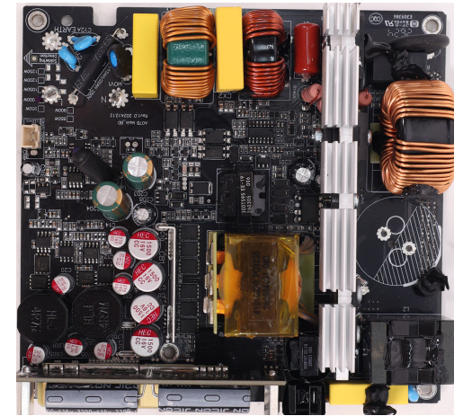
PSU Internals
