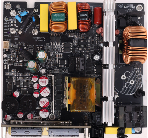
PSU Internals
