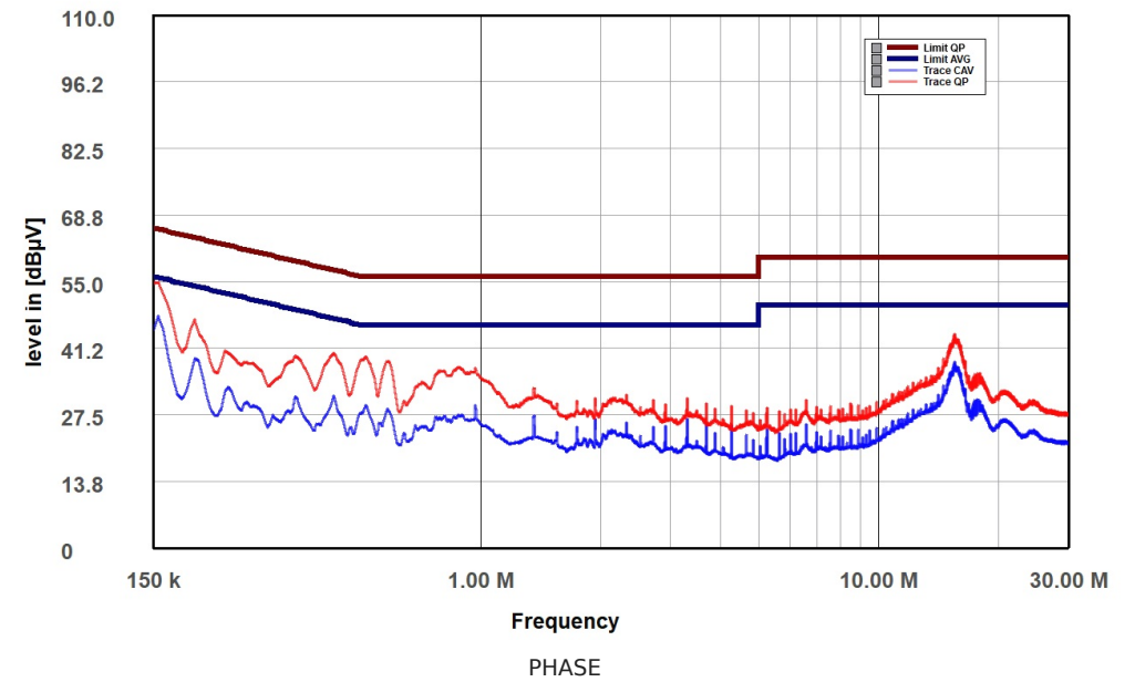
Cooler Master MWE Gold 1000 V4 (CM10003434) Phase
