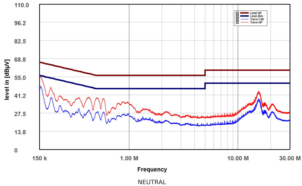
Cooler Master MWE Gold 1000 V4 (CM10003434) Neutral
