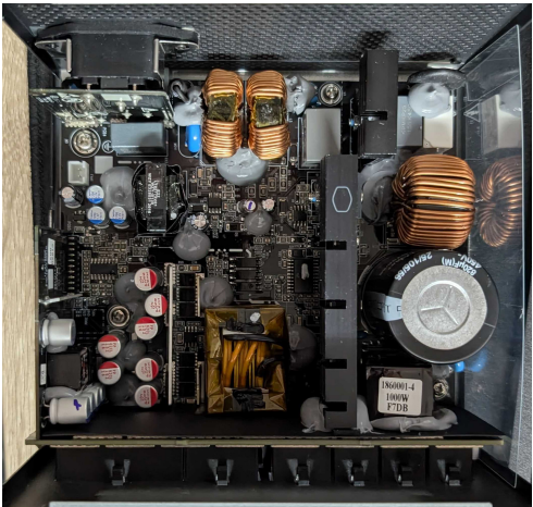
PSU Internals
