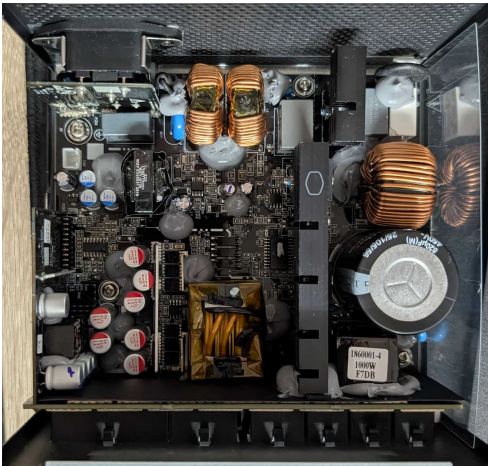
PSU Internals
