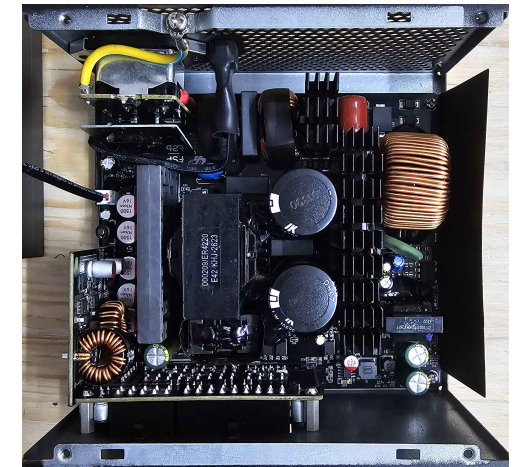
PSU Internals
