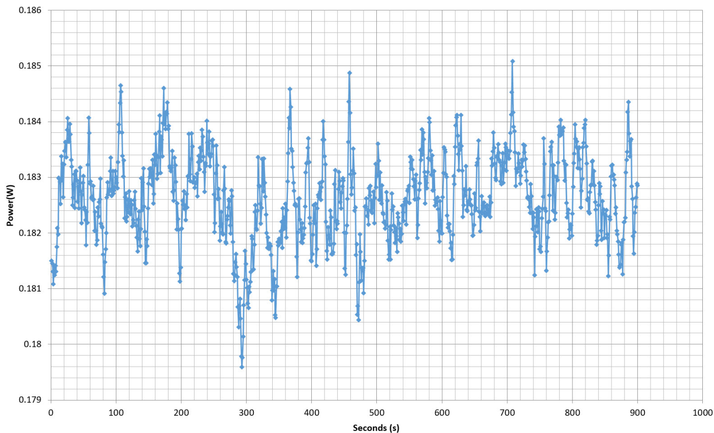
Power - MPE6501ACBW1191400004 - 09/05/2019 - 18:24
