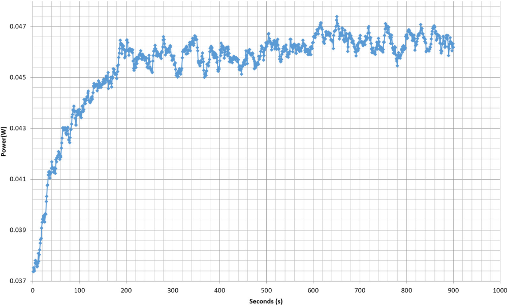
Power - S1908199009 - 19/11/2019 - 11:36
